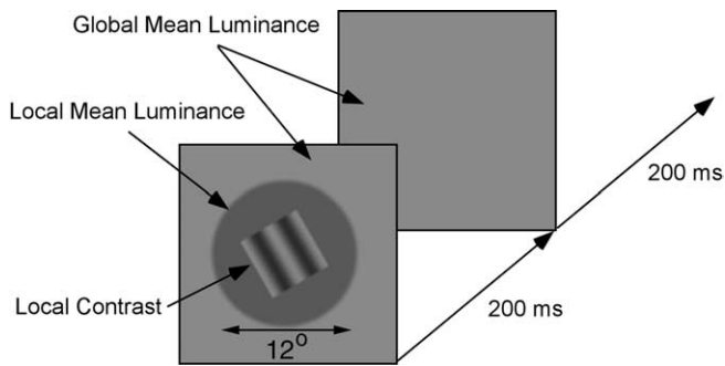
Figure 1. Stimuli for main experiment. In each presentation, a drifting grating stimulus and local mean luminance was displayed for 200 ms (1 cycle of 5 Hz drift), followed by 200 ms of global mean luminance. The local mean luminance and local contrast were parametrically varied and randomly interleaved.
