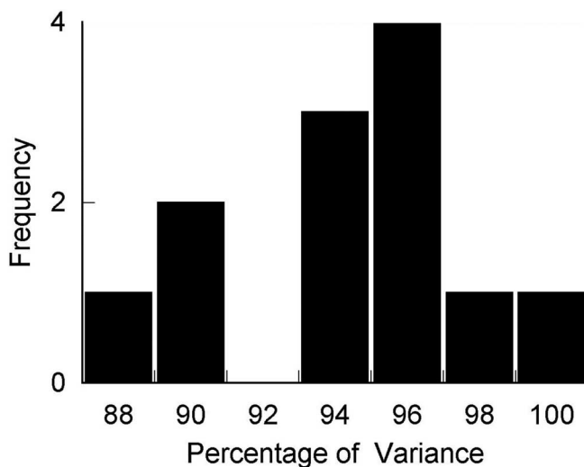
Figure 3. Histogram (across neurons) of the percentage of variance predicted by scaling the average contrast response function separately for each luminance. The good fits indicate that the responses to contrast and luminance are approximately separable.
