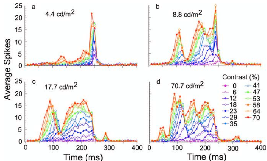
Figure 4. a–d , Temporal response profiles (PSTHs for 10 ms bins) for each combination of transient contrast and transient luminance averaged over 26 experiments on 12 neurons. In agreement with Albrecht et al. (2002), the temporal response profiles are approximately invariant with transient local contrast, up to a scale factor and time shift. However, the temporal response profiles change dramatically with transient luminance and, hence, there appears to be useful information for local mean luminance in the pattern of temporal response.
