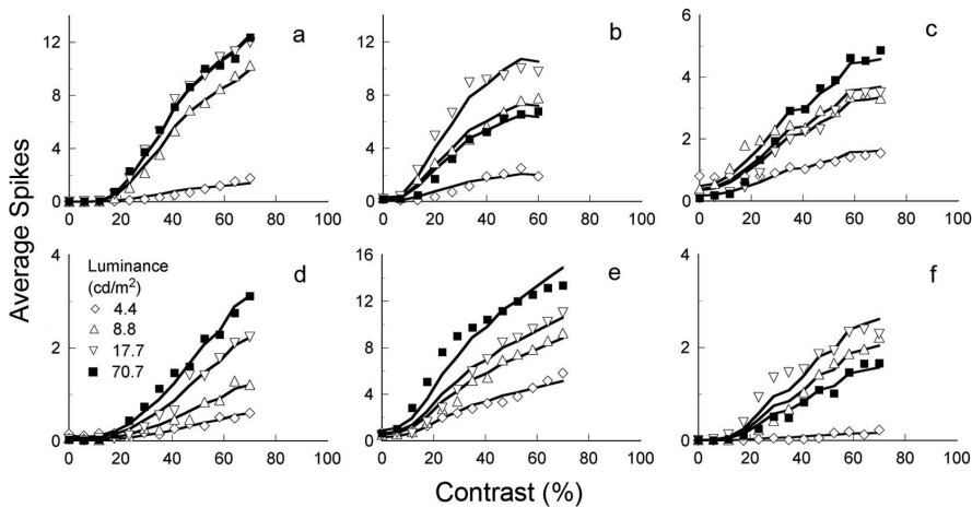
Figure 2. a–f , Responses of six neurons in primary visual cortex of cat to simultaneous transient changes in contrast and luminance. The solid curves are the average contrast response function scaled separately for each luminance. The data in c and e are from complex cells; the data in the other panels are from simple cells.
